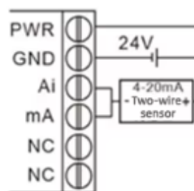
Wiring example of two-wire current sensor
