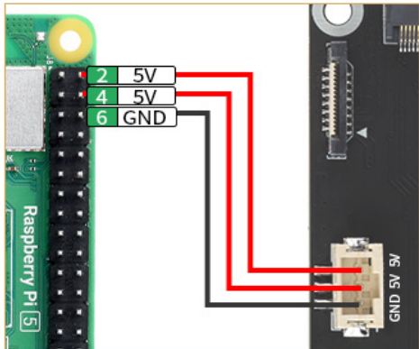
Power supply via 3PIN cable
