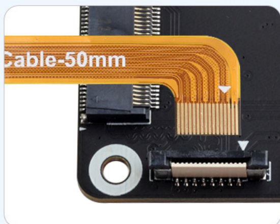
Connect to the PCIe interface of the PCIe TO M.2 Board (C)
